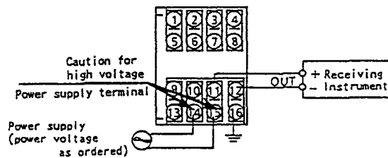
Fig.11 Wiring of Calibration Equipment
