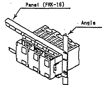
Fig.1 Rack Mounting
