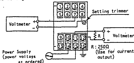
Fig.11 Wiring of Calibration Equipment
